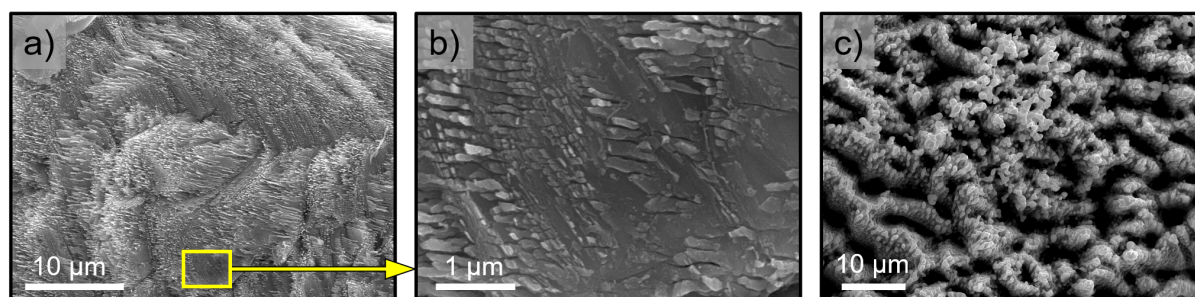
Supplementary Figure S1. SEM photographs of laser-induced periodic structures (LIPS), appeared after multiple passes of WSe 2 crystal surface by femtosecond pulses during ablation experiments; a) Elongated wire-like pattern; b) A magnified area from a), showing the underformed wires pattern; c) Another surface area with low-spatial frequency wavy grooves and high-spatial frequency spherical-like beads.
