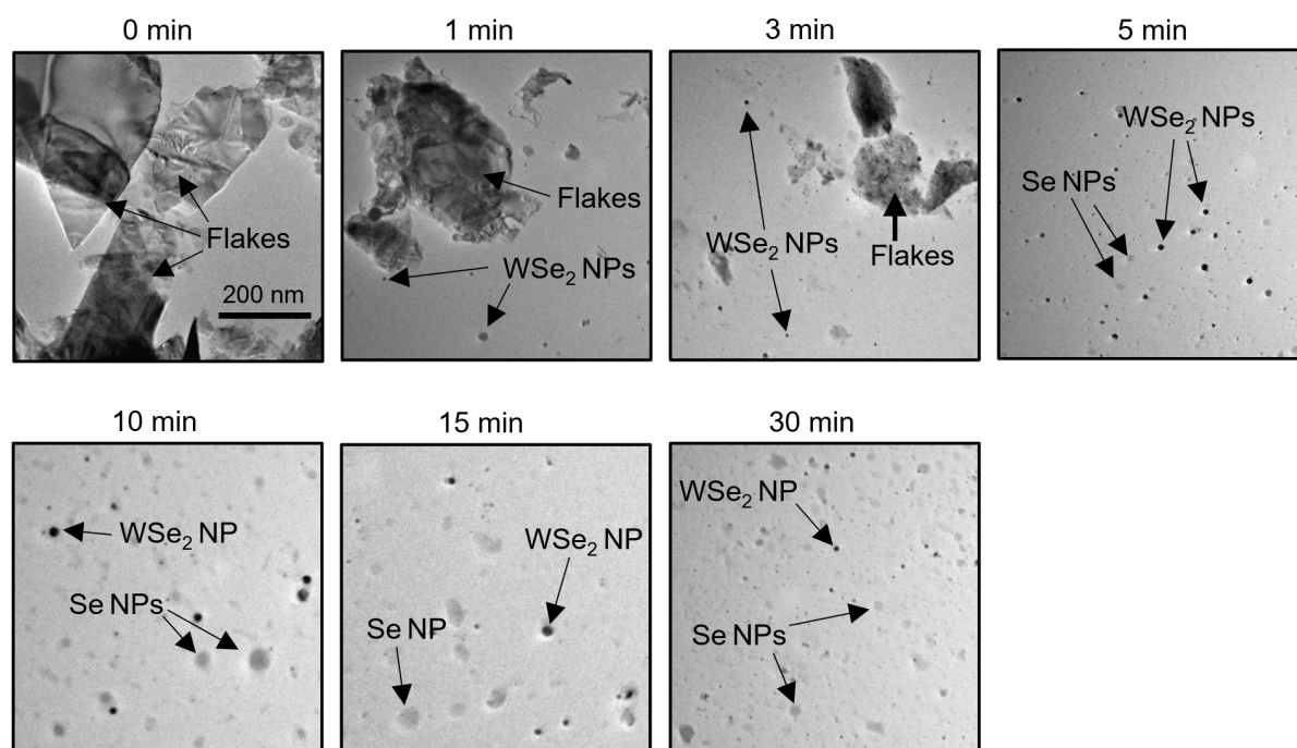
Supplementary Figure S2. TEM photographs of colloids after different time of femtosecond laser fragmentation. At times 5 min and more, Se NPs appear.
